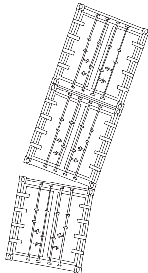
Figure 41.31: Excessive tipping moment or separation force on corner fittings.
