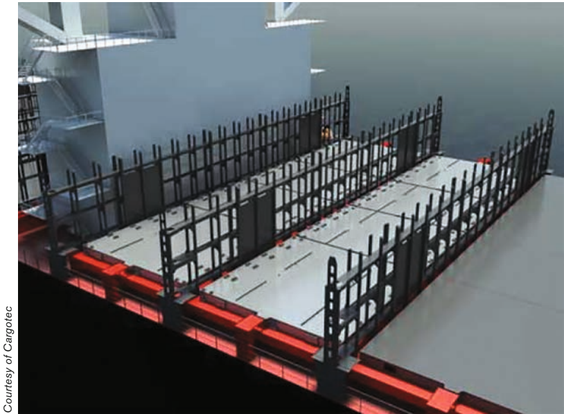
Figure 41.21: Lashing bridges.
