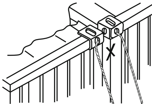
Figure 41.15: Adjacent corner castings should never be loop-lashed.
