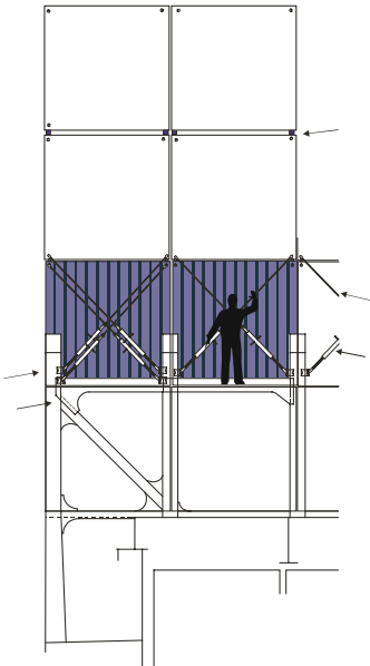
Figure 41.25: Typical post-panamax lashing bridge arrangement (shown 4 high).
