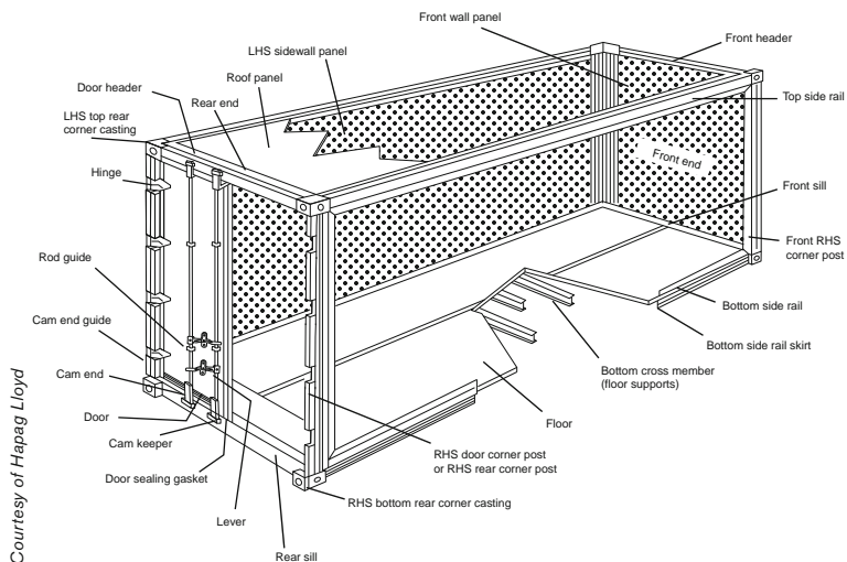
Figure 41.2: Components of a container.
