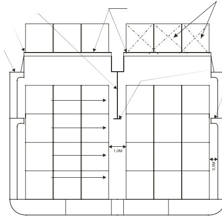
Figure 41.18: Typical midship section of an early vessel conversion.
