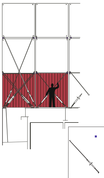
Figure 41.27: Typical container vessel's hatch cover lashing arrangement.
