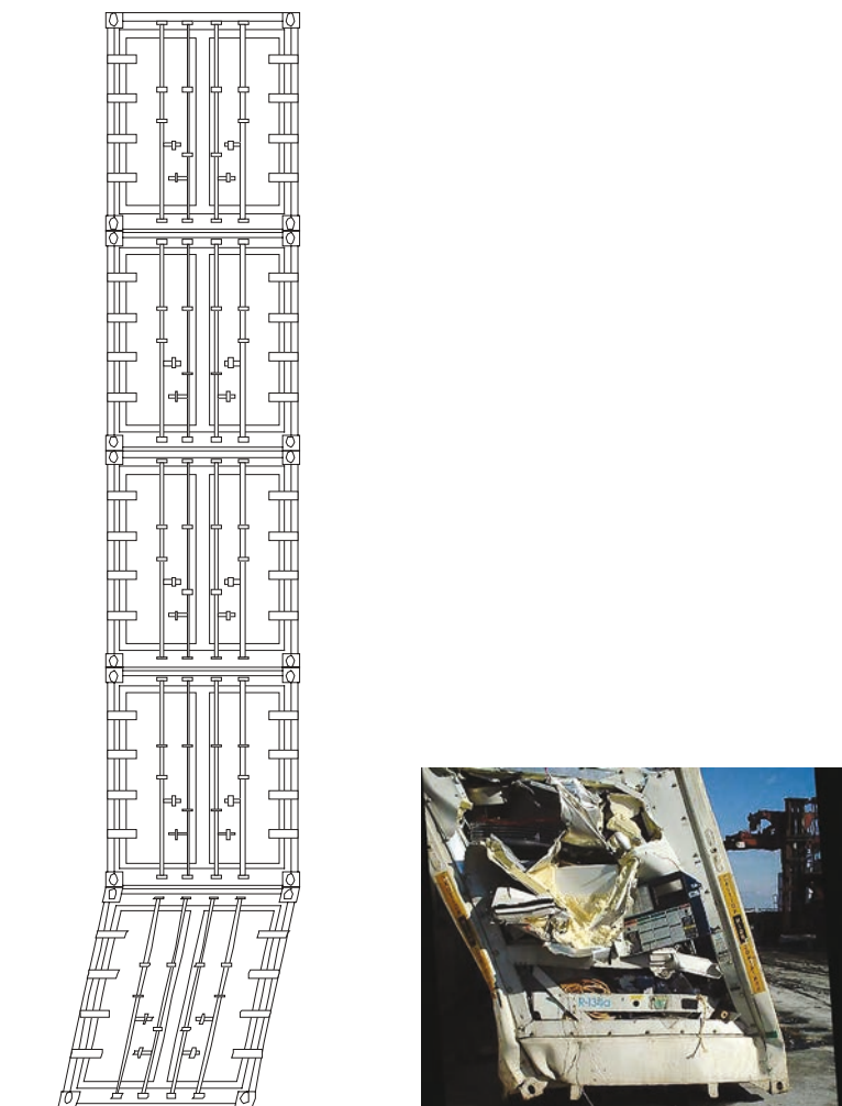
Figure 41.32: Excessive racking force on a container.
