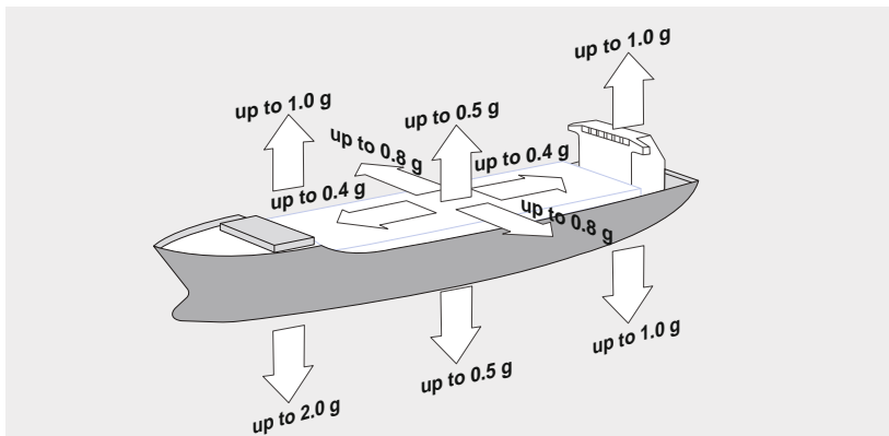
Figure 41.6: Potential accelerations at sea.
