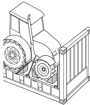
Figure 41.8: Heavy machinery on a 'flat'.
