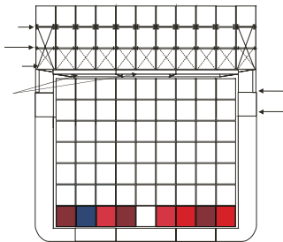
Figure 41.19: Typical midship section of an early generation cellular container vessel.
