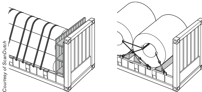
Figure 41.9: Securing points.
