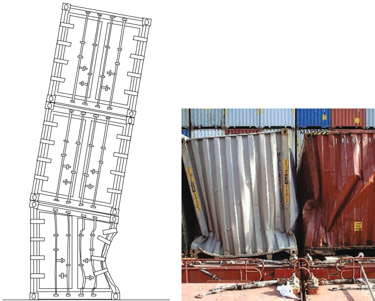
Figure 41.33: Excessive compression force on container corner post, leading to failure of the post.
