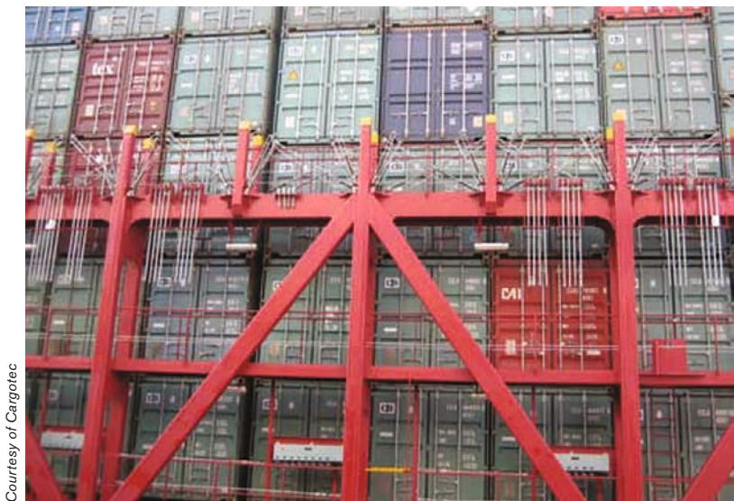
Figure 41.22: Top lashing bridge system for up to 9-high containers.
